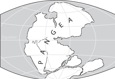
Permian, 225 Myr
