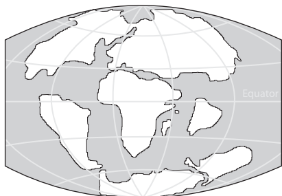
Cretaceous, 65 Myr
