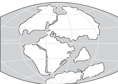
Jurassic, 150 Myr
